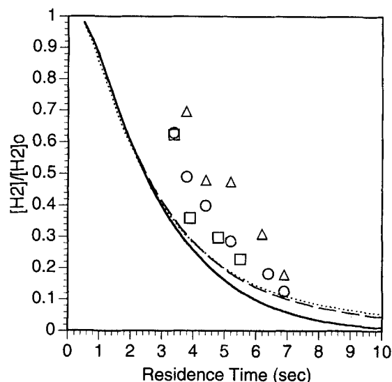
Figure 8. Effect of residence time on H_2 conversion by SCWO at 550°C and [H_2O] = 4.25E-3 \text{ mol/cm}^3 .
