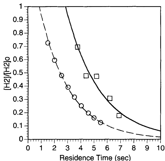
Figure 9. Effect of residence time on \text{H}_2 conversion by SCWO at 550^\circ\text{C} , [\text{H}_2\text{O}] = 4.25\text{E-}3 \text{ mol/cm}^3 , [\text{H}_2]_0 = 3.06\text{E-}6 \text{ mol/cm}^3 , and [\text{O}_2]_0 = 1.55\text{E-}6 \text{ mol/cm}^3 .
